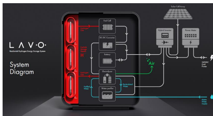
Figures: LAVO 40 kWh Hydrogen Battery and System Diagram, planned for installation at Ularring
